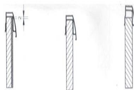
Bútorlap 12 mm + tükör 4 mm Bútorlap 16 mm Bútorlap 18 mm
